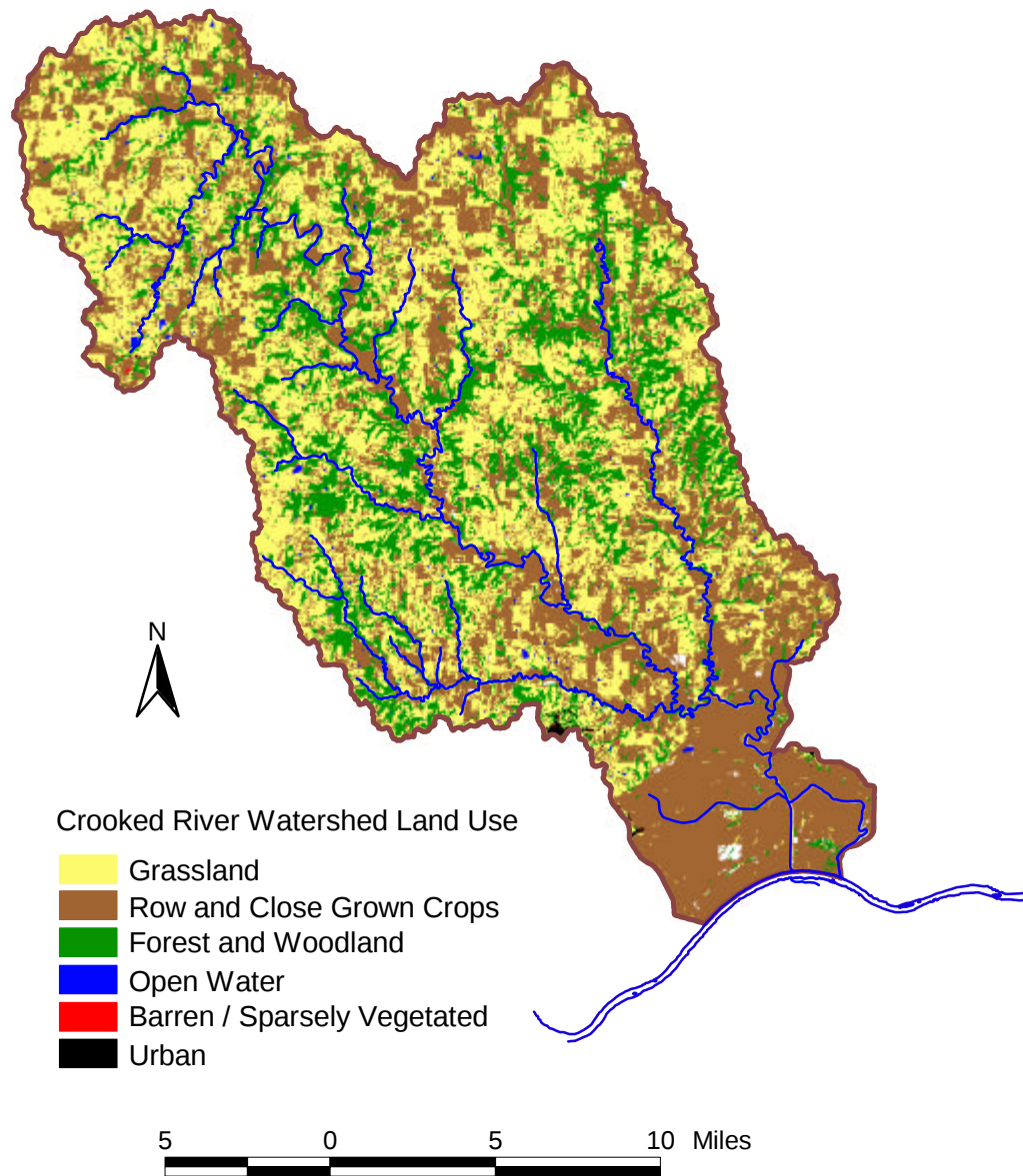
Figure 1u. Land use/land cover within the Crooked River basin (MORAP 1999, preliminary data).
