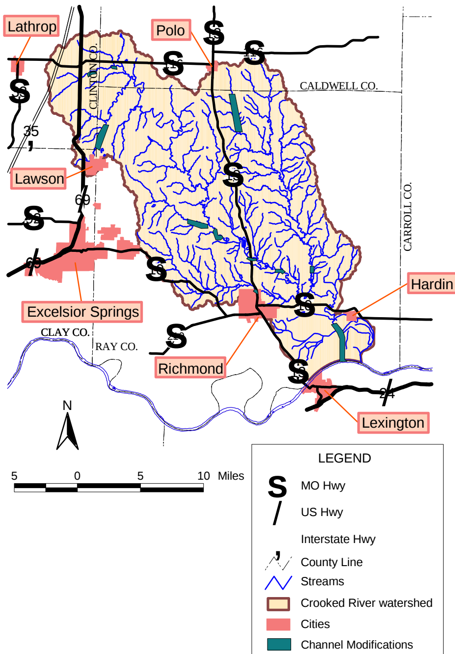
Figure 6. Areas in the Crooked River basin that are noticeably affected by channelization, located using orthophoto quadrangle and topographic maps.
