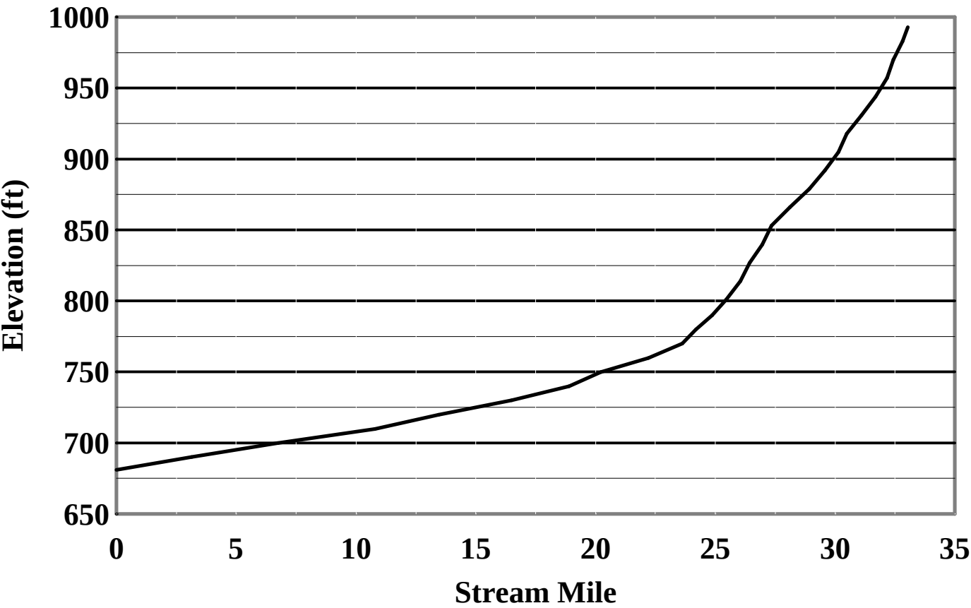
East Fork Crooked River Average Gradient: 9.4 ft/mi
