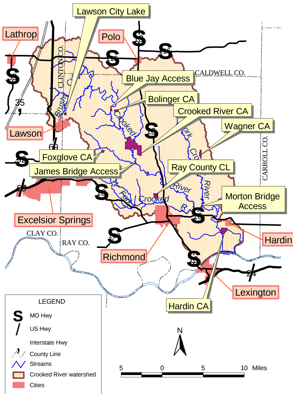
Figure 2. Public land within the Crooked River basin.
