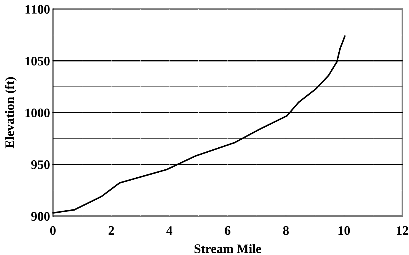
Stevenson Creek Average Gradient: 17.1 ft/mi
