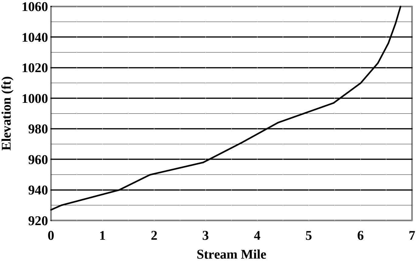
Unnamed #32 Average Gradient: 19.6 ft/mi
