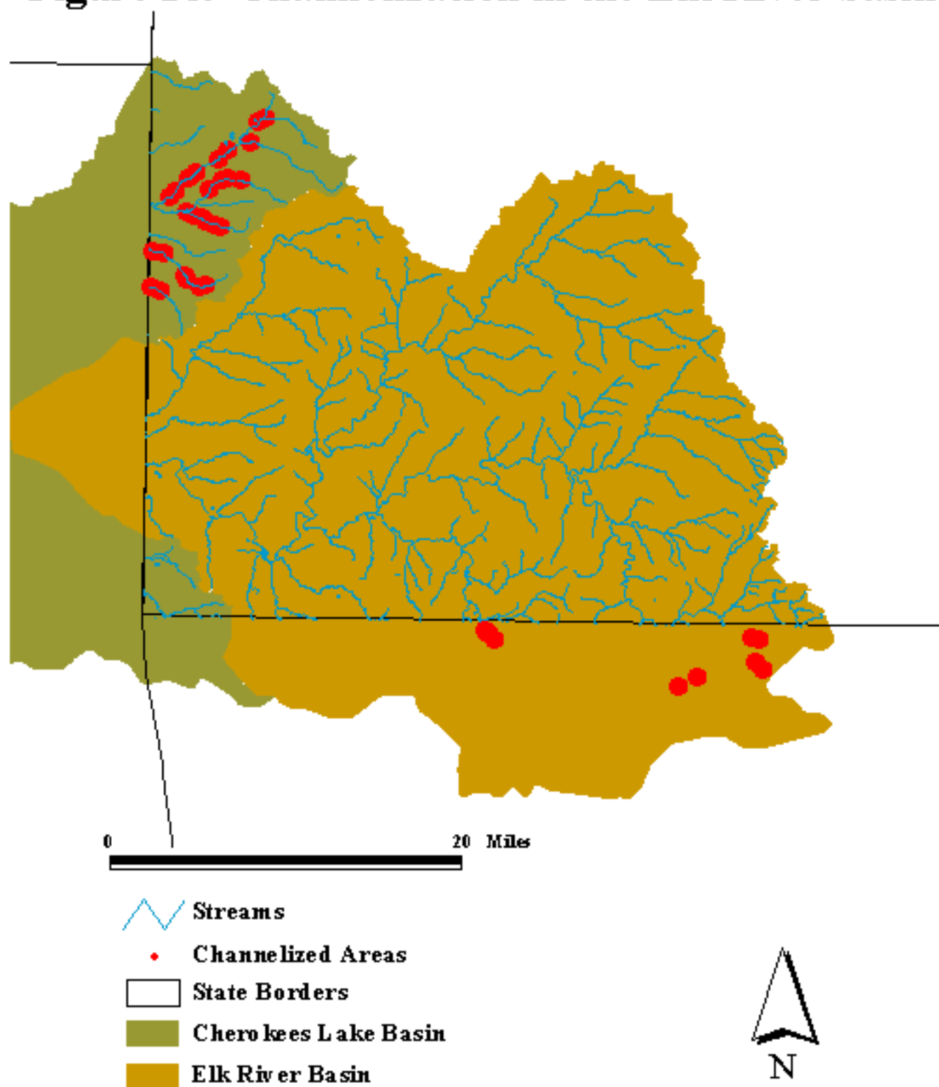
Figure 18. Channelization in the Elk River basin.
