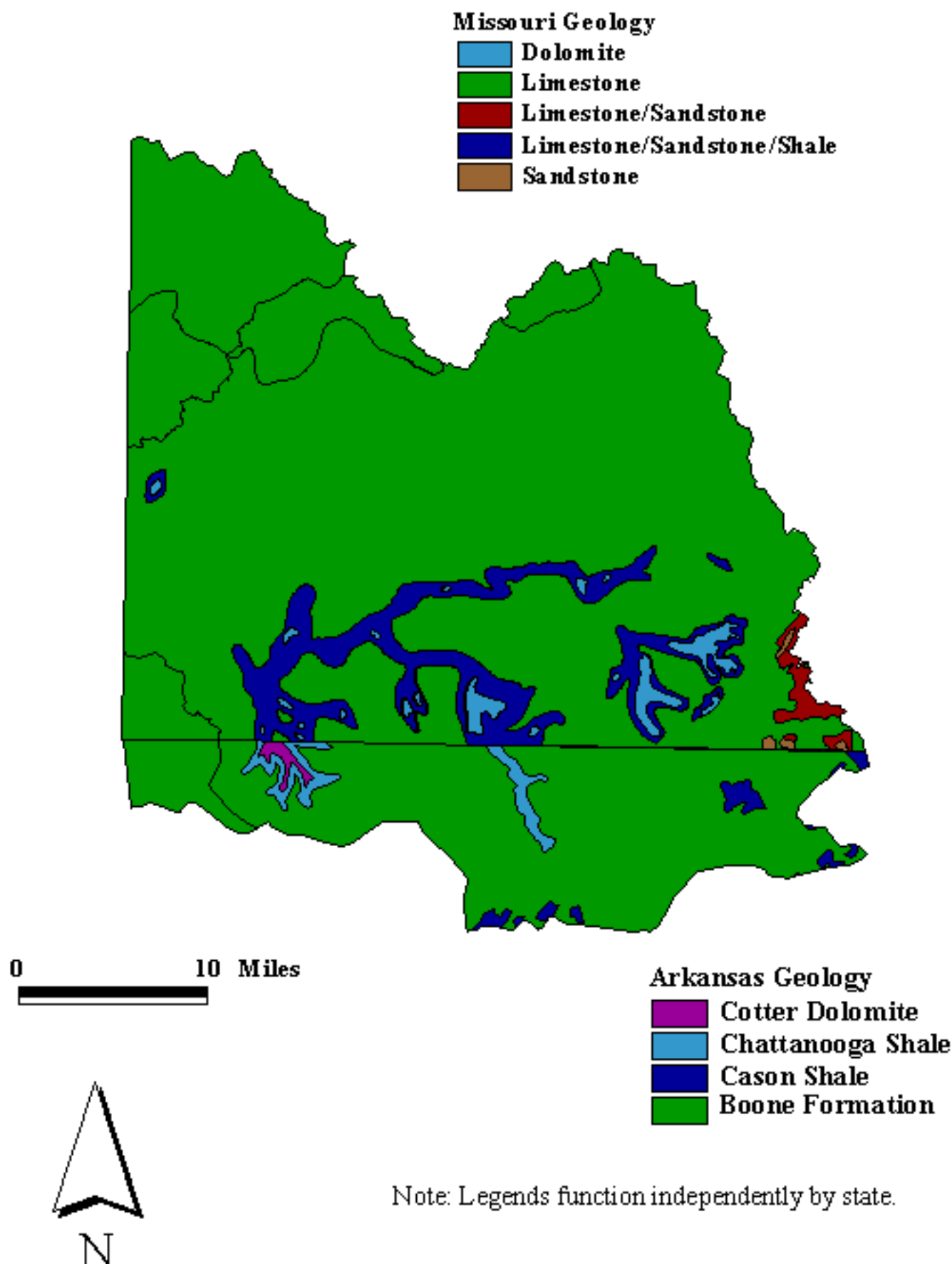
Figure 07. Elk River basin geology.
