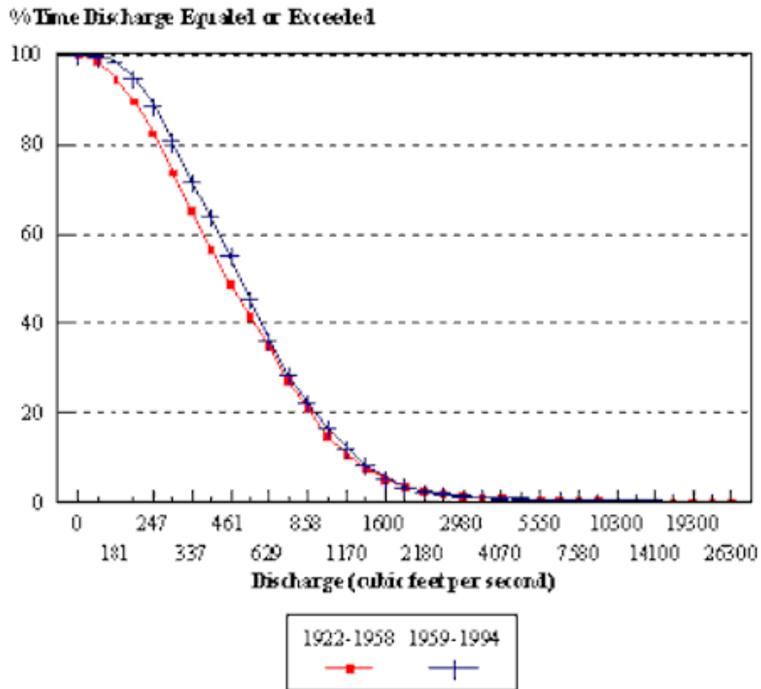
Figure H-06. Flow duration changes between two time periods for the Eleven Point River near Bardley (USGS 1995).
