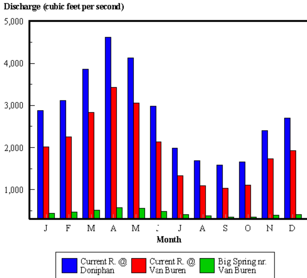
Figure Hy04. Monthly mean daily discharge at selected USGS Gage Stations within the Current River Watershed (USGS 2000b).
